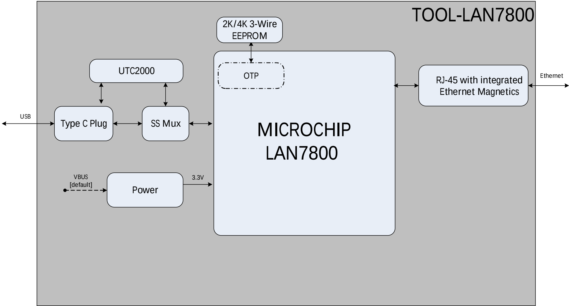
EVB Floor Plan
