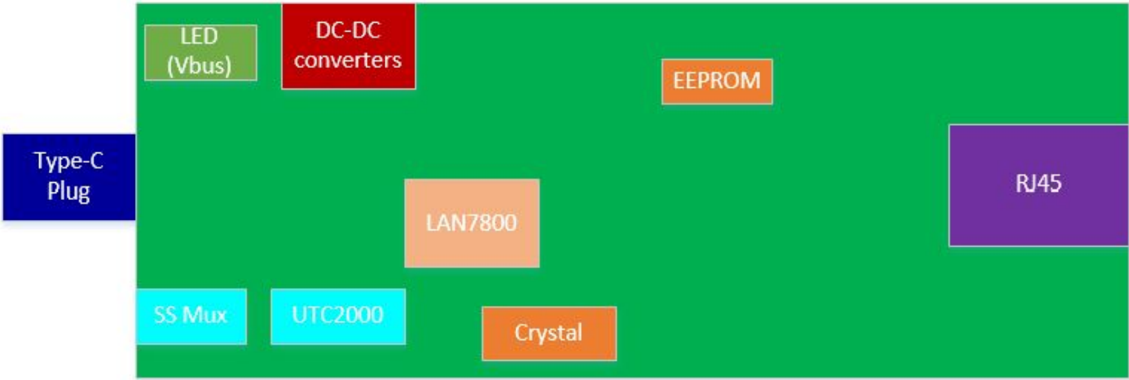
EVB Floor Plan
